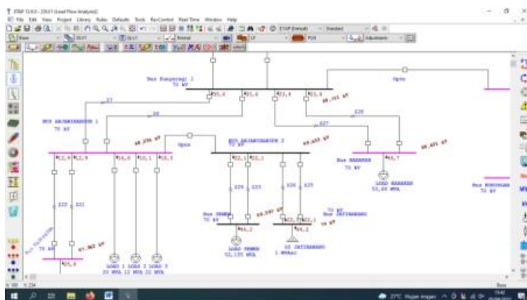
Gambar 6, Tegangan bus 1 Sunyaragi keadaan normal
