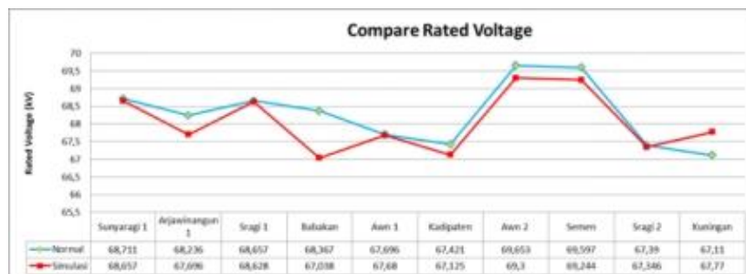
Gambar 16 Grafik Compare Rated Voltage
