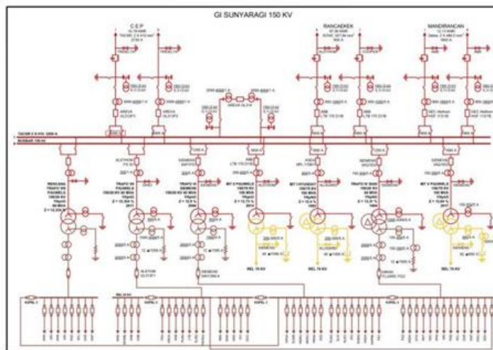
Gambar 1, Single Line Diagram sistem 150 kV
